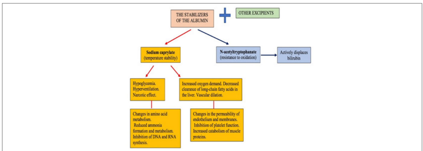
Figure 2: The main stabilizers of albumin, their role and influence.
