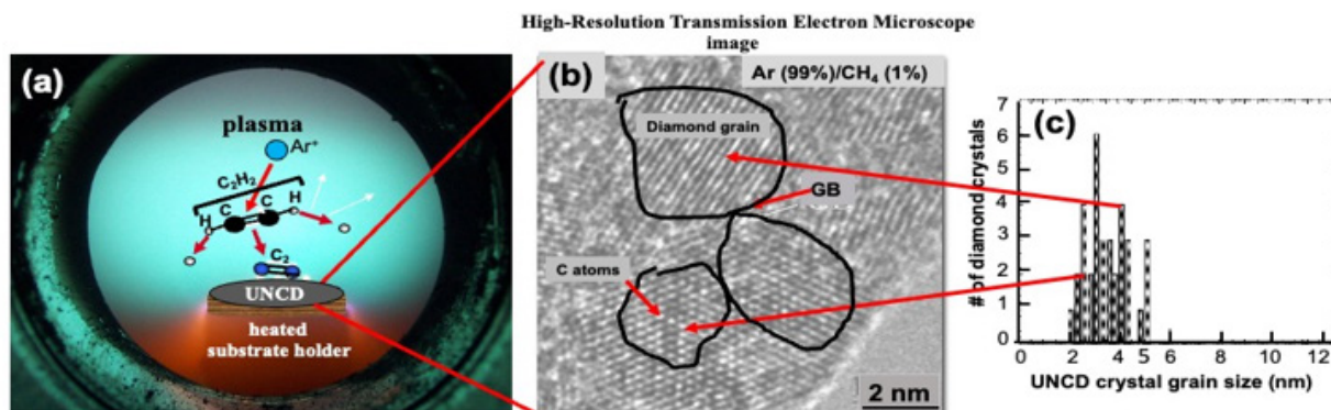
Figure 1: (a) Picture of microwave plasma created via excitation of Ar (99%)/CH 4 (1%) gas mixture (the schematic shows Ar ions producing the key C 2 dimers that initiate the UNCD films' nucleation and subsequent growth, jointly with CH x (x= 1, 2, 3) molecules created in the plasma, all reacting on the substrate's surface); (b) High Resolution Transmission Electron Microscopy (HRTEM) image of a UNCD film grown on a silicon substrate (the white dots are C atoms in diamond crystal lattice positions in the grain); (c) UNCD grain dimensions measured via HRTEM.
